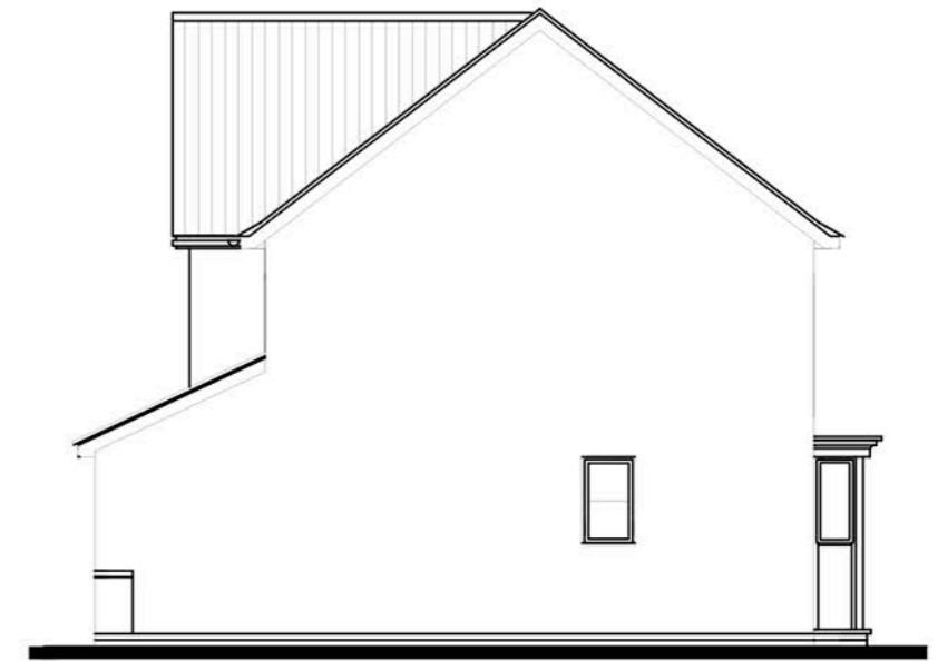
SIDE ELEVATION Derwent
